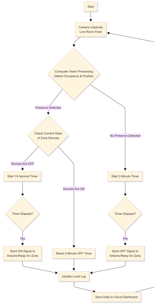
Fig. 2. Room-level operational workflow showing live video capture, local inference, zoning-based control decisions, and relay-based appliance actuation.
